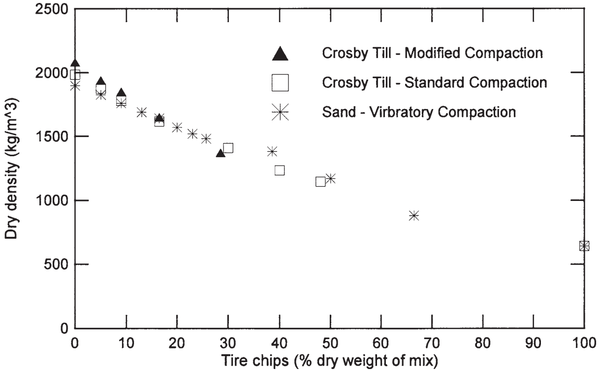
FIG. X1.1 Comparison of Compacted Dry-Density of Mixtures of Tire Shreds with Ottawa Sand and Crosby Till (5)
